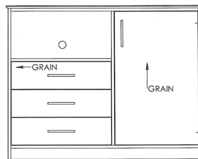
F-DU-DB-B223 Microfridge 54 x 24 x 42 F-DU-DB-B223C Microfridge w/Door 54 x 24 x 42
